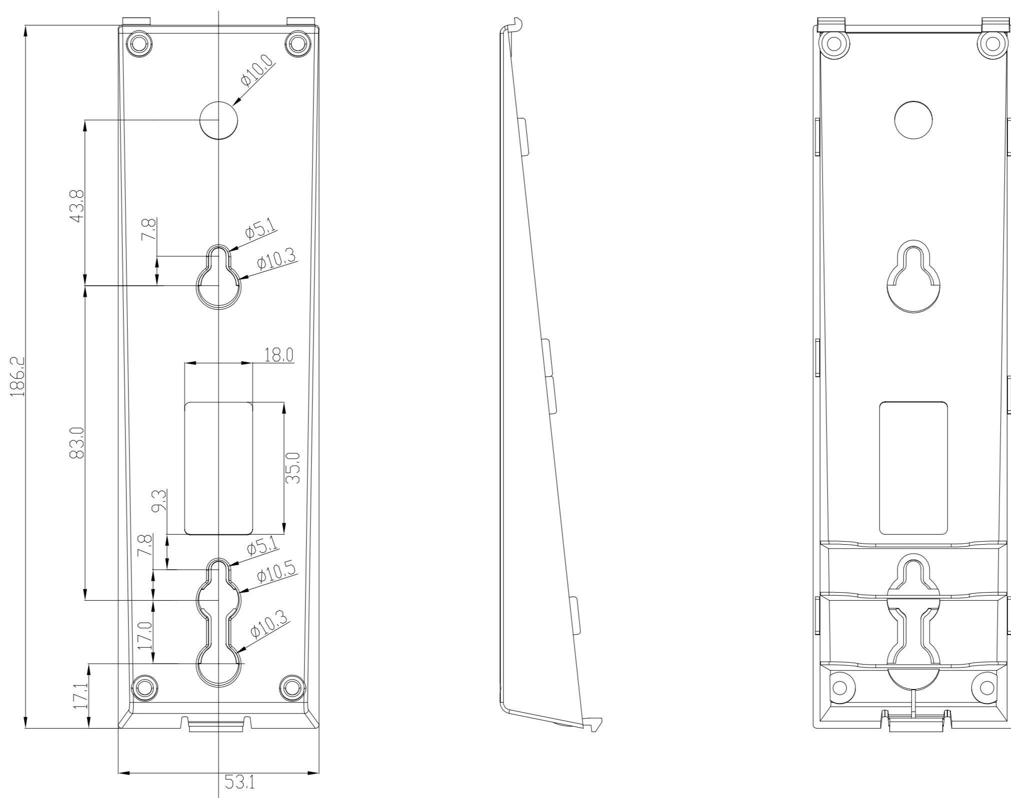
Single Drawing (Scale 1:1)
