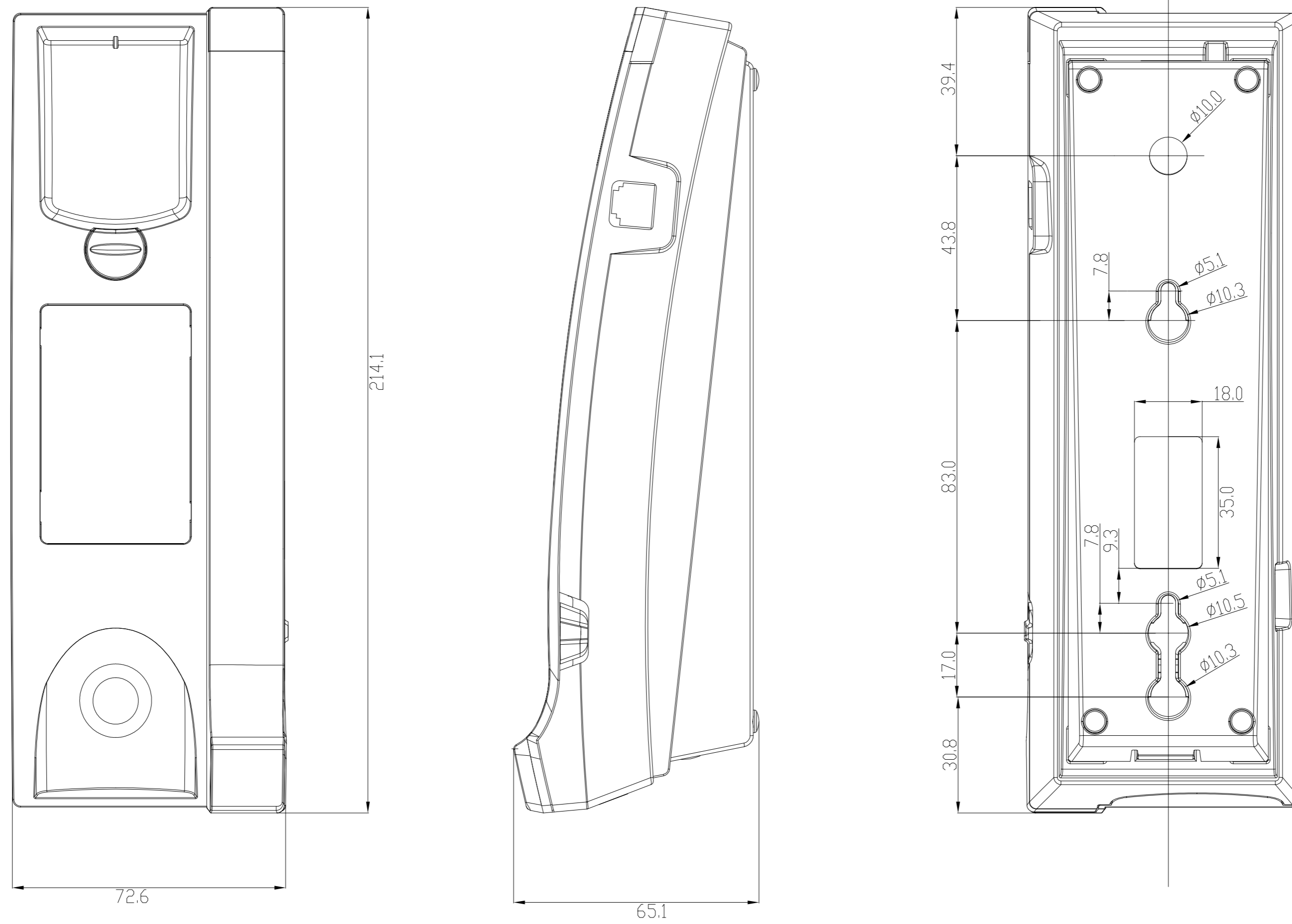
Assembly Drawing (Scale 1:1)
