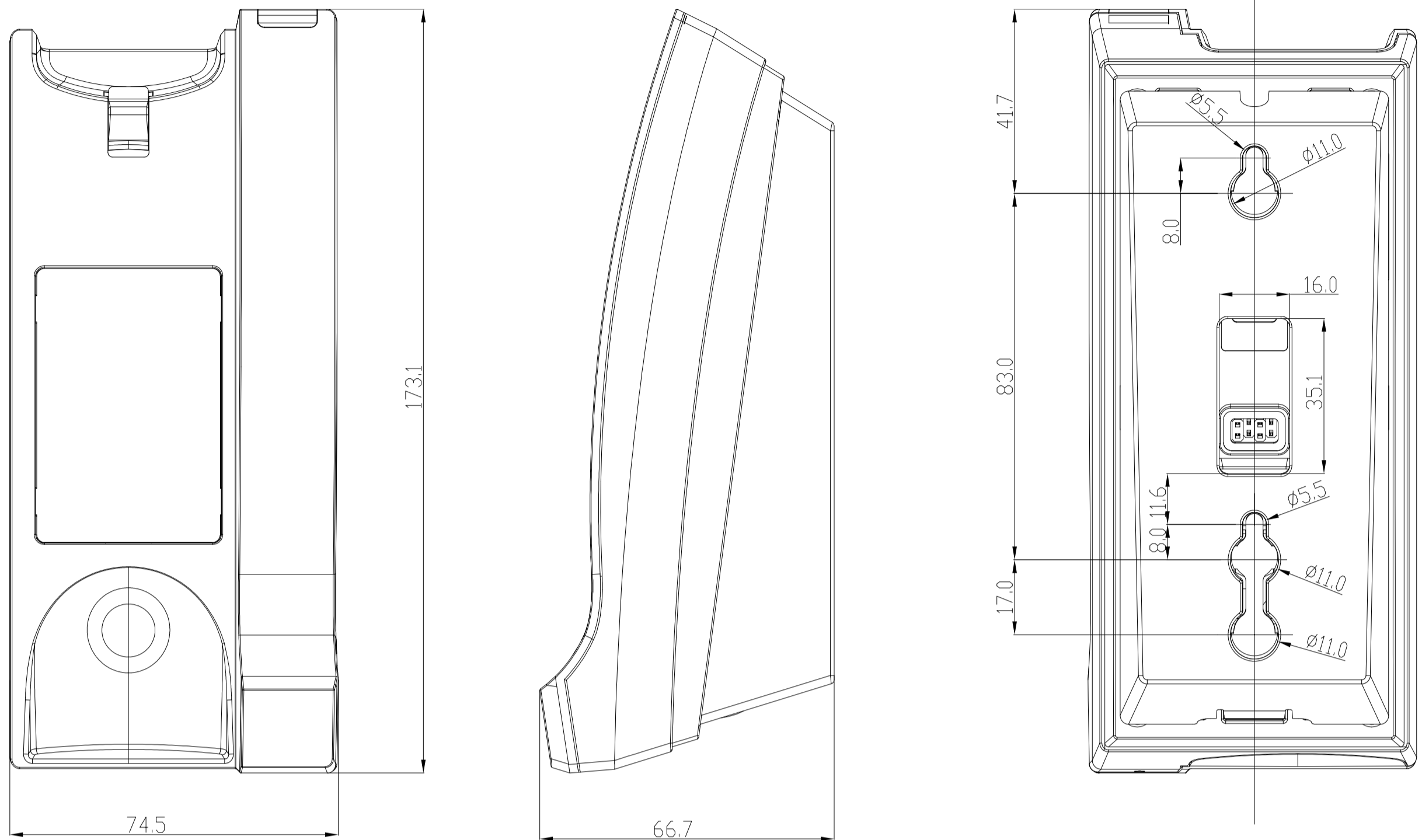
Assembly Drawing (Scale 1:1)
